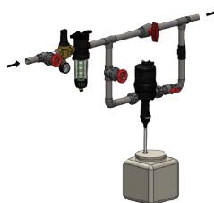
bypass installation
