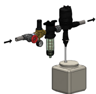
inline installation
